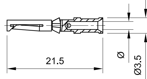
Female contact
