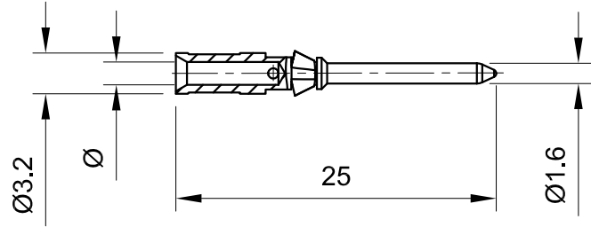
Male contact
